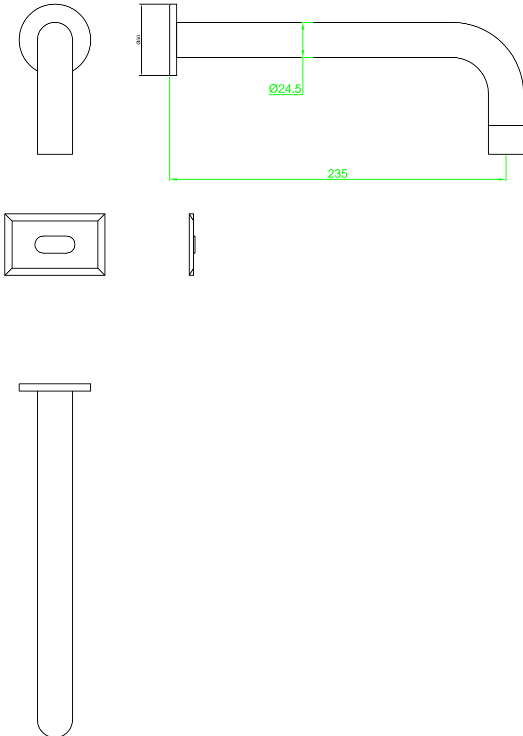
WALL AUTOMATIC FAUCET MF-120
